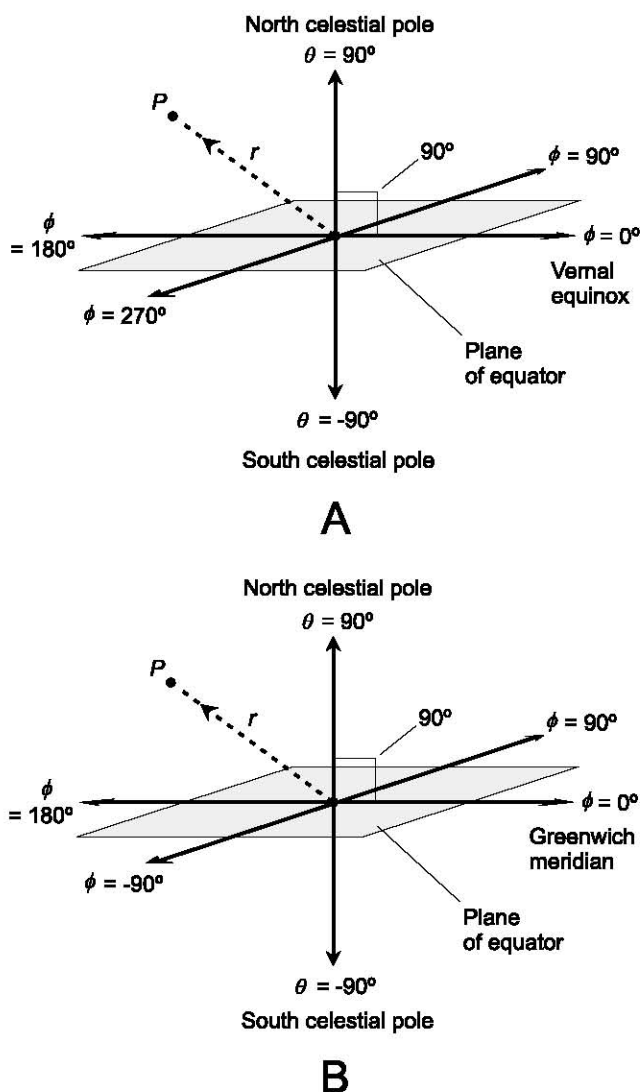
Fig. 6-4. (A) Spherical coordinates for defining points in three-space, where the angles \theta and \phi represent declination and right ascension, and r represents radius or range. (B) Spherical coordinates for defining points in three-space, where the angles \theta and \phi represent latitude and longitude, and r represents radius or range.
